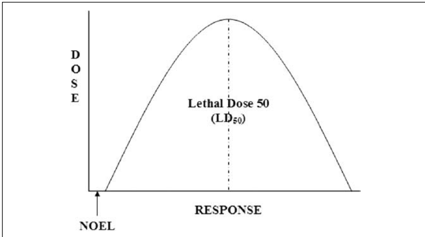
Figure 6-2. The dose-response relationship.
