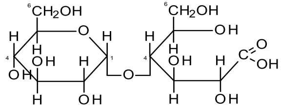
maltobionic acid
