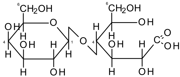
lactobionic acid
