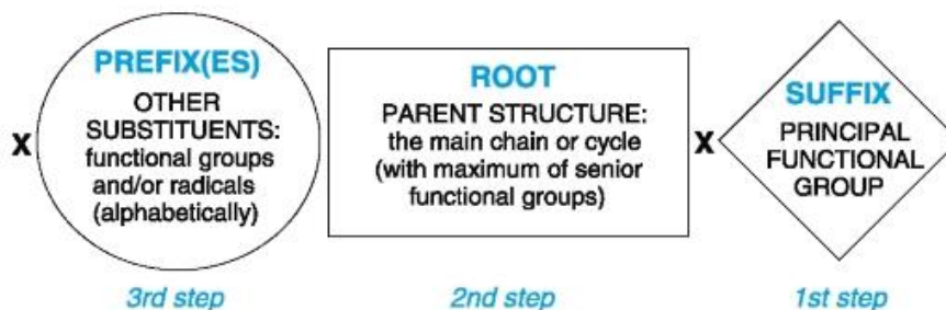
Figure 1. The scheme for constructing the IUPAC substitutive name. The symbol \times represents multiplying affix(es).
