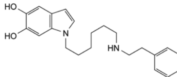
K. 1-[6-[(2-phenylethyl)amino]hexyl]-1H-indole-5,6-diol.
