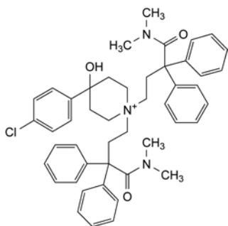
B. 4-(4-chlorophenyl)-1,1-bis[4-(dimethylamino)-4-oxo-3,3-diphenylbutyl]-4-hydroxypiperidinium,
