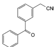
I. (3-benzoylphenyl)ethanenitrile,
