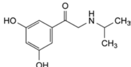
B. 1-(3,5-dihydroxyphenyl)-2-[(1-methylethyl)amino]ethanone,
