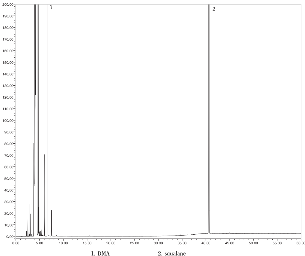
Figure 1630.-1. – Chromatogram of squalane of animal origin
