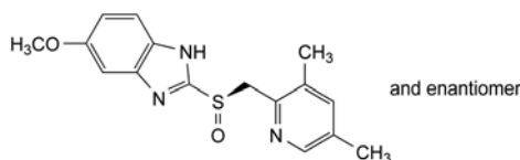
B. 2-[(RS)-[(3,5-dimethylpyridin-2-yl)methyl]sulfinyl]-5-methoxy-1H-benzimidazole,
