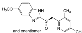
B. 2-[(RS)-[(3,5-dimethylpyridin-2-yl)methyl]sulfinyl]-5-methoxy-1H-benzimidazole,
