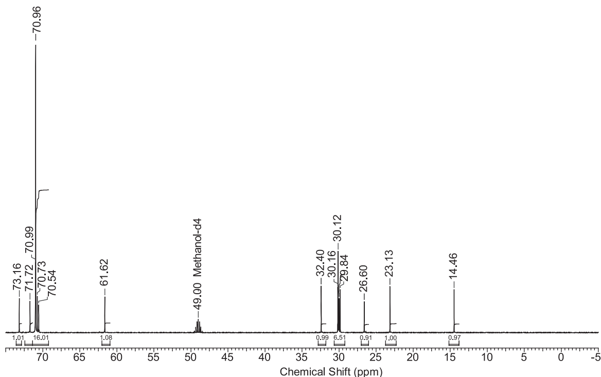
Figure 2046.-1. - 13 C NMR spectrum of lauromacrogol 400
