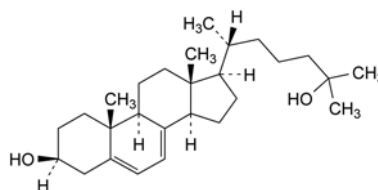
B. cholesta-5,7-diene-3β,25-diol,
