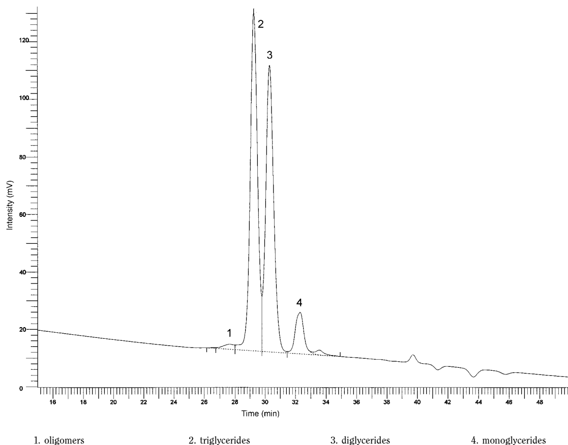
Figure 1352.-1. – Chromatogram for the test for oligomers and partial glycerides
