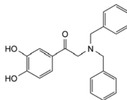
G. 2-(dibenzylamino)-1-(3,4-dihydroxyphenyl)ethanone.
