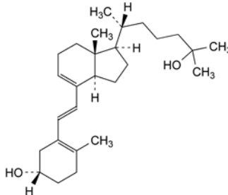
C. (6E)-9,10-secocholesta-5(10),6,8-triene-3β,25-diol,
