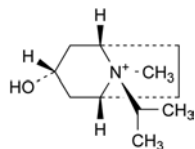
A. (1R,3r,5S,8r)-3-hydroxy-8-methyl-8-(1-methylethyl)-8-azoniabicyclo[3.2.1]octane,
