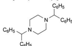
E. 1,4-bis(diphenylmethyl)piperazine.
