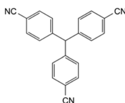
B. 4,4',4''-methanetriyltribenzonitrile.
