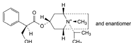
B. (1R,3r,5S,8s)-3-[(2RS)-3-hydroxy-2-phenylpropanoyl]oxy-8-methyl-8-(1-methylethyl)-8-azoniabicyclo[3.2.1]octane,
