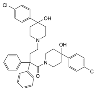
E. 4-(4-chlorophenyl)-1-[4-[4-(4-chlorophenyl)-4-hydroxypiperidin-1-yl]-2,2-diphenylbutanoyl]piperidin-4-ol,
