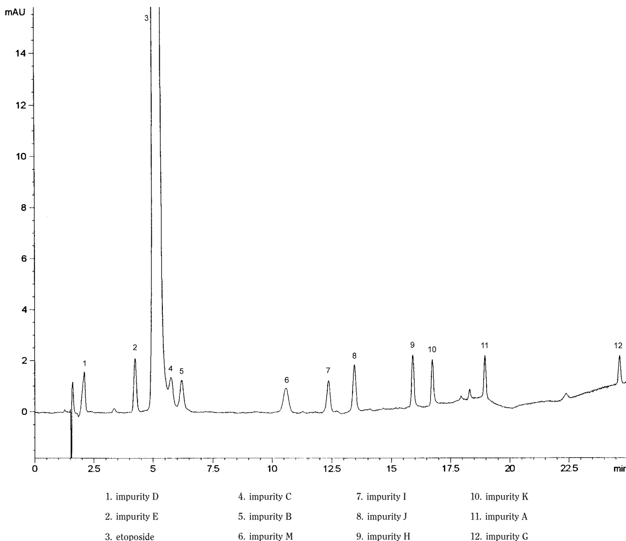
Figure 0823-1. – Chromatogram for the test for related substances of etoposide
