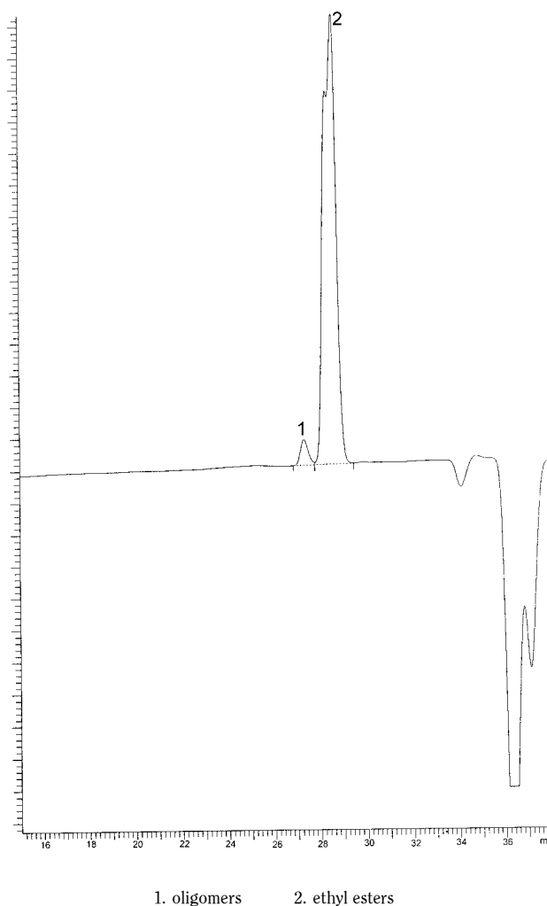
Figure 1250.-1. – Chromatogram for the test for oligomers: spiked sample
