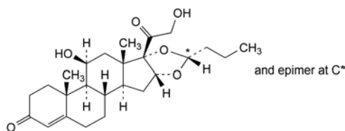
G. 16α,17-[(1RS)-butylidenebis(oxy)]-11β,21-dihydroxypregna-4-ene-3,20-dione.
