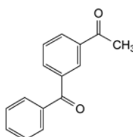
A. 1-(3-benzoylphenyl)ethanone,
