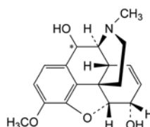
E. 7,8-didehydro-4,5α-epoxy-3-methoxy-17-methylmorphinan-6α,10-diol,
