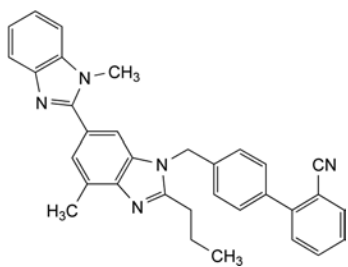
G. 4'-[[4-methyl-6-(1-methyl-1H-benzimidazol-2-yl)-2-propyl-1H-benzimidazol-1-yl]methyl]biphenyl-2-carbonitrile,
