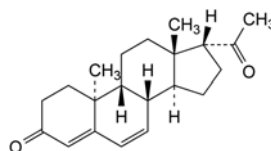
C. 9β,10α,17α-pregna-4,6-diene-3,20-dione.
