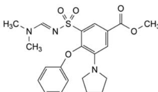
B. methyl-3-[[[dimethylamino]methylene]sulfamoyl]-4-phenoxy-5-(pyrrolidin-1-yl)benzoate,
