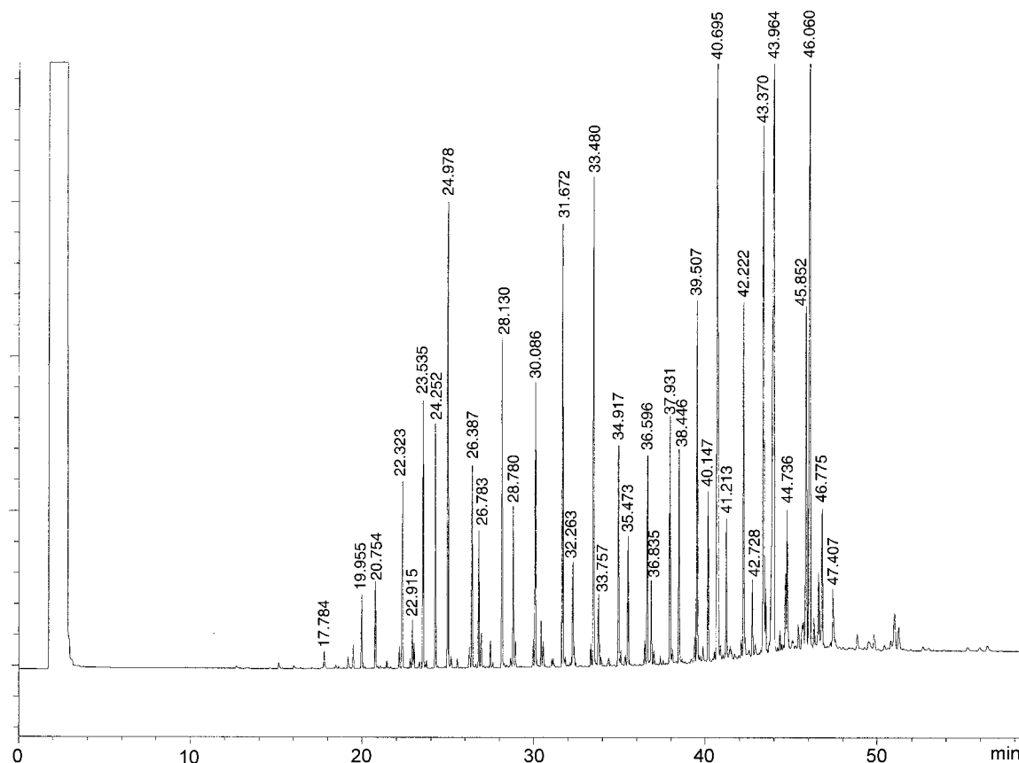
Figure 0969.-1. – Chromatogram for the test for fatty alcohols and sterols (reference solution (a)) in hydrogenated wool fat
