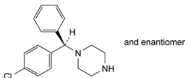
H. 1-[(RS)-(4-chlorophenyl)phenylmethyl]piperazine.
