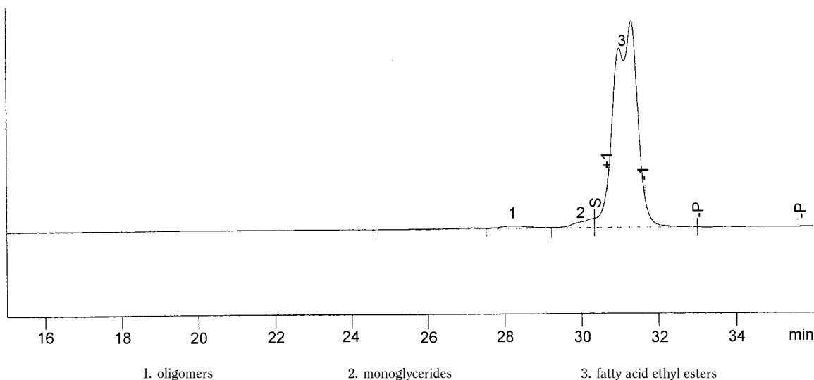
Figure 2063-1. – Chromatogram for the test for oligomers and partial glycerides
