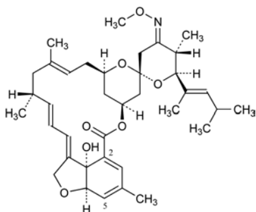
H. 2,5-didehydro-5-deoxymoxidectin,
