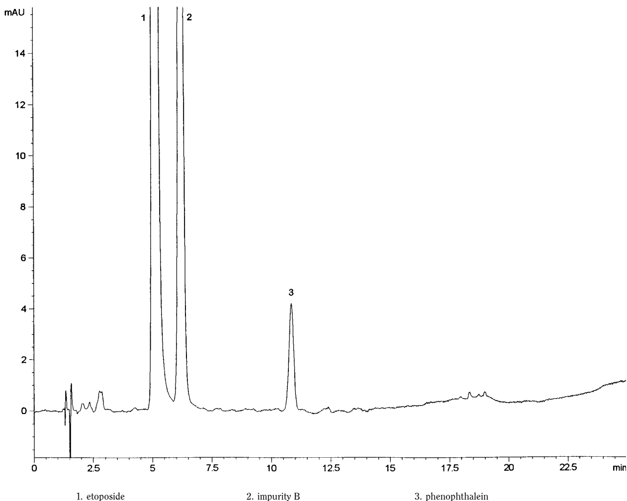
Figure 0823.-2. - Chromatogram for the test for related substances of etoposide: reference solution (d)
