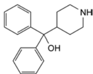
I. diphenyl(piperidin-4-yl)methanol.
