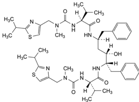
T. (2S)-N-[(1S,2S,4S)-1-benzyl-2-hydroxy-4-[[2-(2S)-3-methyl-2-[[methyl][2-(1-methylethyl)thiazol-4-yl]methyl]carbamoyl]amino]butanoyl]amino]-5-phenylpentyl]-3-methyl-2-[[methyl][2-(1-methylethyl)thiazol-4-yl]methyl]carbamoyl]amino]butanamide,
