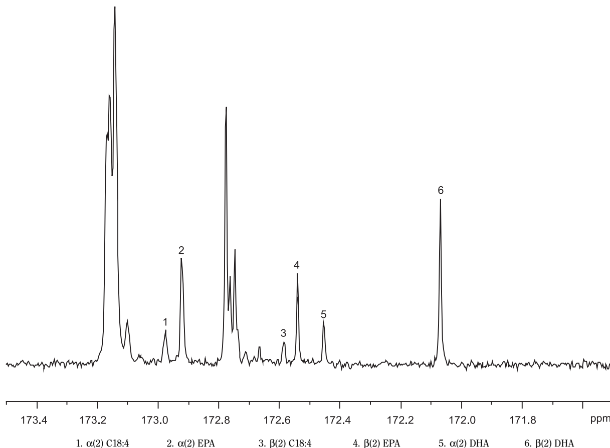
Figure 2398.-1. – 13 C NMR spectrum carbonyl region of farmed cod-liver oil
