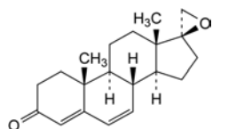
H. (2'S)-spiro[androst-4,6-diene-17,2'-oxiran]-3-one,
