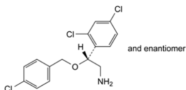
B. (2RS)-2-[(4-chlorobenzyl)oxy]-2-(2,4-dichlorophenyl)ethanamine,
