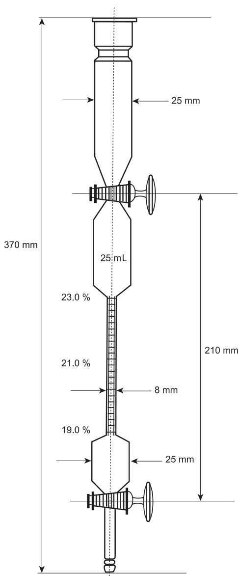
Figure 1238.-2. – Gas burette
