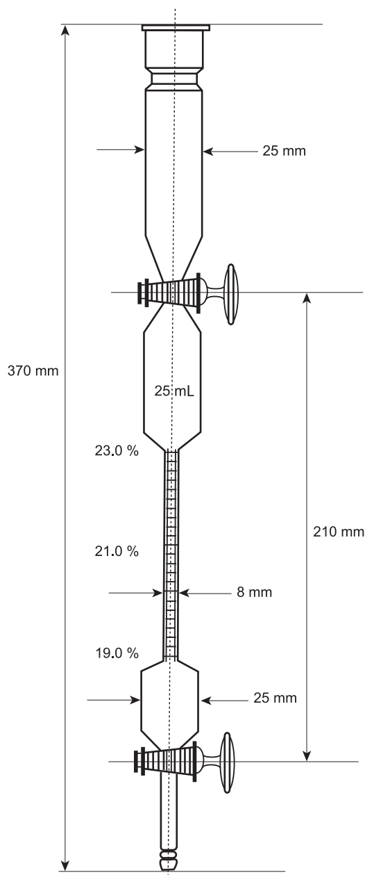
Figure 1684-1.- Gas burette
