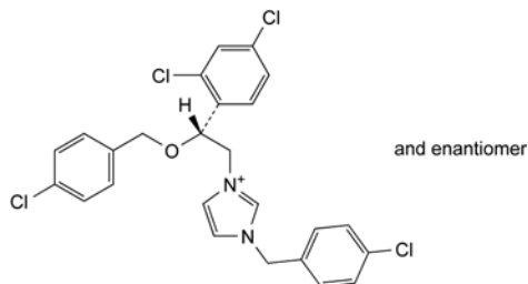
C. 1-(4-chlorobenzyl)-3-[(2RS)-2-[(4-chlorobenzyl)oxy]-2-(2,4-dichlorophenyl)ethyl]imidazolium.
