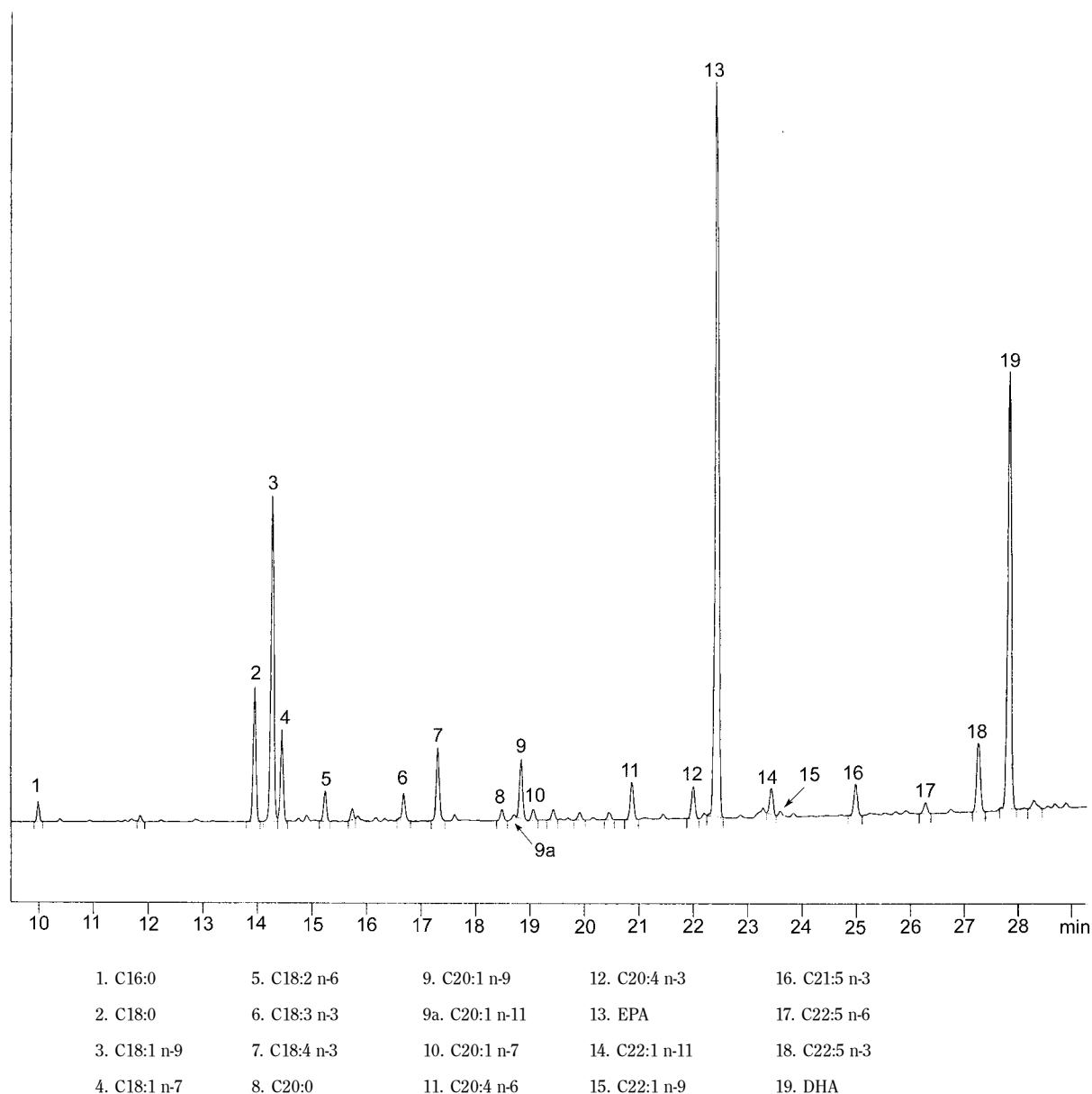
Figure 2063.-2. – Chromatogram for the assays
