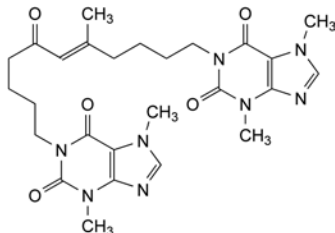
J. 1-[(5E)-11-(3,7-dimethyl-2,6-dioxo-2,3,6,7-tetrahydro-1H-purin-1-yl)-5-methyl-7-oxoundec-5-enyl]-3,7-dimethyl-3,7-dihydro-1H-purine-2,6-dione.
