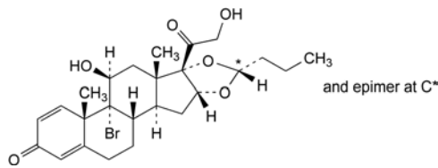
J. 16α,17-[(1RS)-butylidenebis(oxy)]-9α-bromo-11β,21-dihydroxypregna-1,4-diene-3,20-dione,
