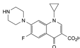
B. ciprofloxacin,
