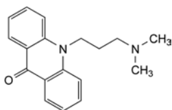
C. 10-[3-(dimethylamino)propyl]acridin-9(10H)-one.
