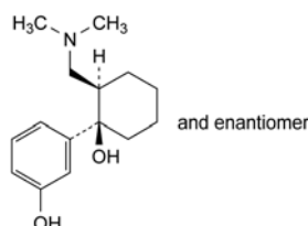
D. (1RS,2RS)-2-[(dimethylamino)methyl]-1-(3-hydroxyphenyl)cyclohexanol,
