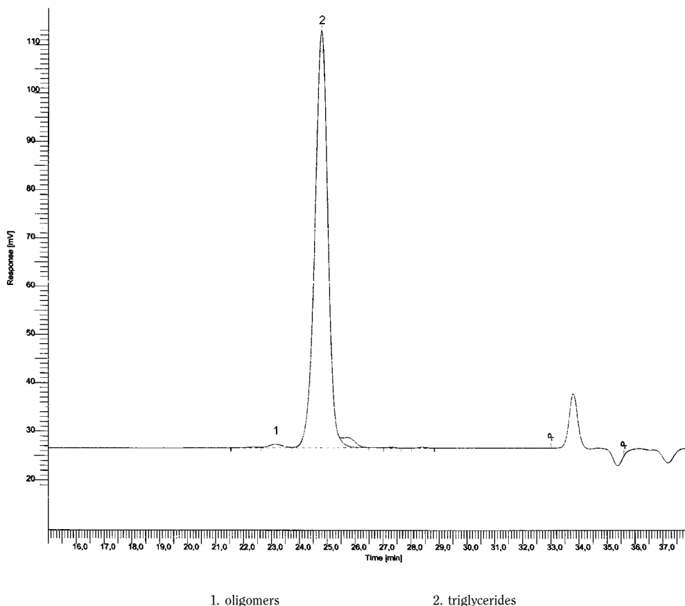
Figure 1912.-1. – Chromatogram for the test for oligomers in fish oil rich in omega-3 acids
