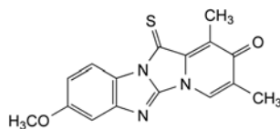
F. 8-methoxy-1,3-dimethyl-12-thioxopyrido[1',2':3,4]imidazo[1,2-a]benzimidazol-2(12H)-one,
