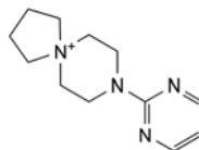
B. 8-(pyrimidin-2-yl)-8-aza-5-azoniaspiro[4.5]decane,
