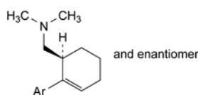
C. (1RS)-[2-(3-methoxyphenyl)cyclohex-2-enyl]-N,N-dimethylmethanamine,
