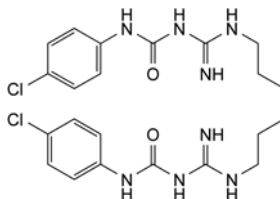
C. 1,1'-[hexane-1,6-diylbis(iminocarbonimidoyl)]bis[3-(4-chlorophenyl)urea],
