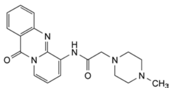
C. 6-[[[4-methylpiperazin-1-yl]acetyl]amino]-11H-pyrido[2,1-b]quinazolin-11-one,
