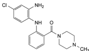
D. 1-[2-[(2-amino-4-chlorophenyl)amino]benzoyl]-4-methylpiperazine.
