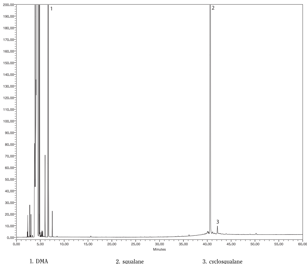
Figure 1630.-2. – Chromatogram of squalane of vegetable origin
