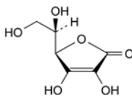
F. (5R)-5-[(1R)-1,2-dihydroxyethyl]-3,4-dihydroxyfuran-2(5H)-one,
