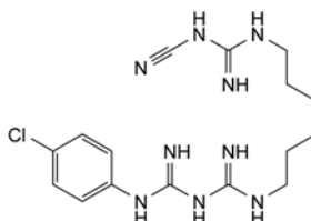
A. 1-(4-chlorophenyl)-5-[6-[(cyanocarbamimidoyl)amino]hexyl]biguanide,
