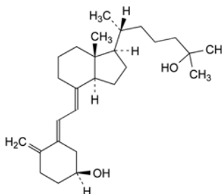
D. (5E,7E)-9,10-secocholesta-5,7,10(19)-triene-3β,25-diol.
