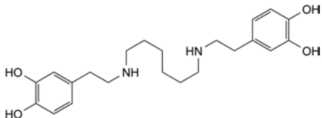
A. 4,4'-[hexane-1,6-diylbis(iminoethylene)]dibenzene-1,2-diol,
