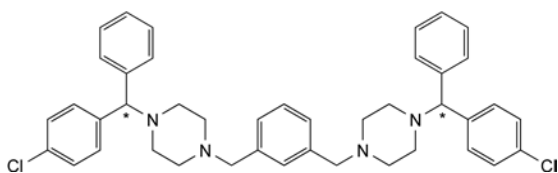
D. 1,1'-(1,3-phenylenebismethylene)bis[4-[(4-chlorophenyl)phenylmethyl]piperazine],
