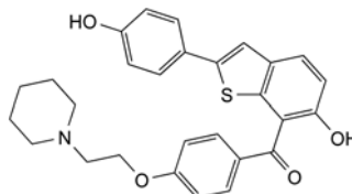
B. [6-hydroxy-2-(4-hydroxyphenyl)-1-benzothiophen-7-yl][4-[2-(piperidin-1-yl)ethoxy]phenyl]methanone,
