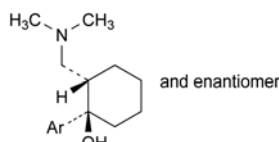
A. (1RS,2SR)-2-[(dimethylamino)methyl]-1-(3-methoxyphenyl)cyclohexanol,
