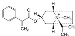
F. (1R,3r,5S,8r)-8-methyl-8-(1-methylethyl)-3-[(2-phenylpropenoyl)oxy]-8-azoniabicyclo[3.2.1]octane.
