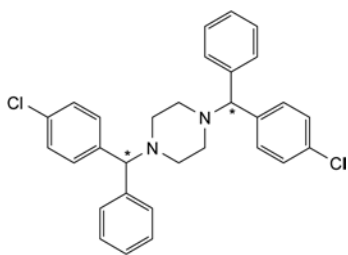
D. 1,4-bis[(4-chlorophenyl)phenylmethyl]piperazine.
