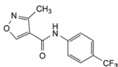
E. 3-methyl-N-[4-(trifluoromethyl)phenyl]isoxazole-4-carboxamide.
