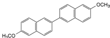
F. 6,6'-dimethoxy-2,2'-binaphthalenyl.
