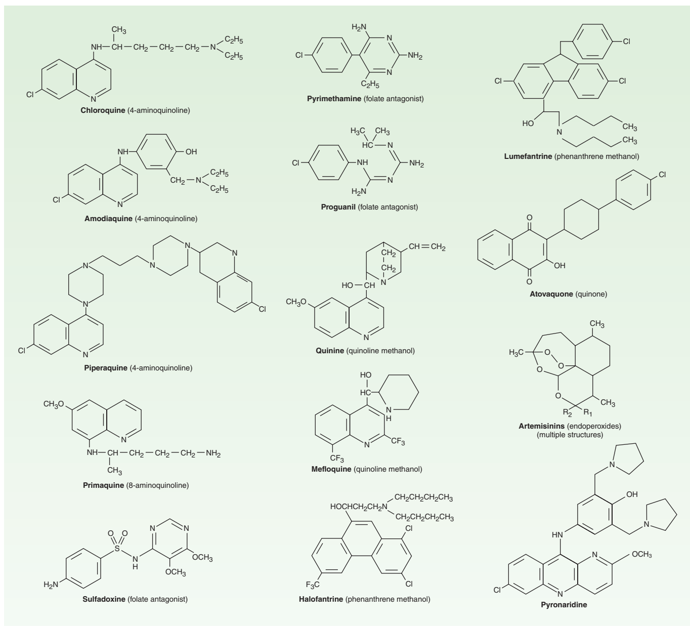
FIGURE 52-2 Structural formulas of some antimalarial drugs.
