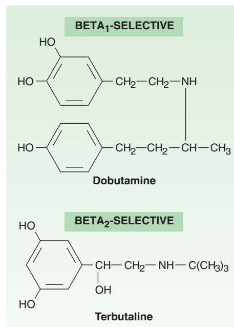
FIGURE 9–8 Examples of \beta_1 - and \beta_2 -selective agonists.
