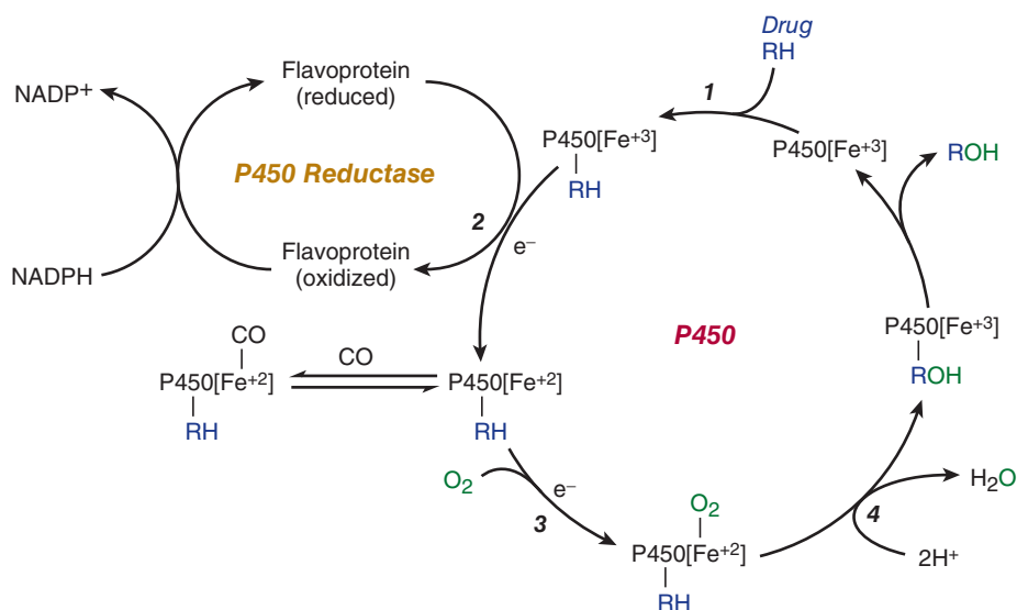
FIGURE 4-3 Cytochrome P450 cycle in drug oxidations. \text{e}^- , electron; RH, parent drug; ROH, oxidized metabolite.
