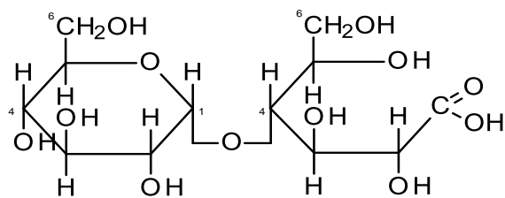
maltobionic acid
