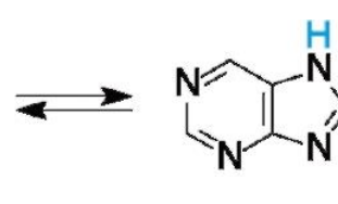
7H-purine
