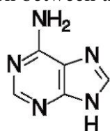
adenine
