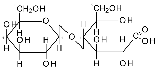
lactobionic acid
