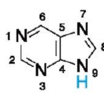
9H-purine
