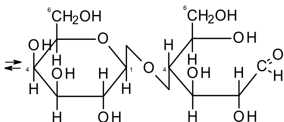
D-lactose
